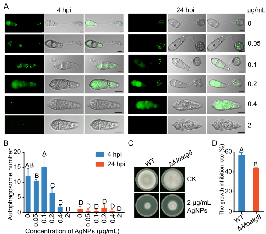
Fig. 4 Conidial autophagy is repressed by AgNPs. A. Conidial autophagy was monitoring by the marker protein GFP-Atg8 using confocal microscopy during appressorium development. Conidial drops supplemented with different concentrations of 2 nm-AgNPs were inoculated on hydrophobic plastic surfaces to induce appressoria formation. Images were taken at the indicated time points 4 and 24 hpi. Bar, 5 µm. B. The numbers of autophagosomes in conidia. More than 20 conidia were counted each time. C. The deletion mutant \Delta Moatg8 showed lower sensitivity to 2 nm-AgNPs than that of the WT. D. The growth inhibition rates of WT and \Delta Moatg8 cultured on CM plates amended with 2 µg mL -1 AgNPs. Photographs were taken at 6 dpi.
