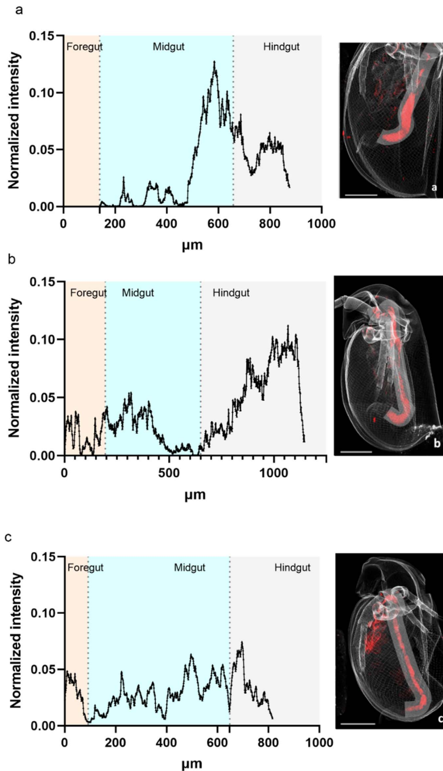
Fig. 6 Variation of La normalized intensity along the intestinal tract of daphnids exposed for 48 h ((a) organism Fig. 2a) and for 72 h ((b) organism Fig. 2b and c, organism Fig. 2c). Line of 90 \mu\text{m} width. Beamline: NANOSCOPIUM. Incident energy of 17.02 keV.
