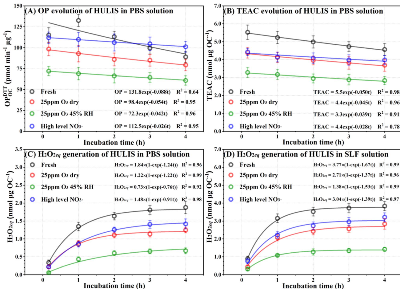
Fig. 5 Evolution of (A) OP, (B) TEAC, and (C) H 2 O 2eq generation for fresh and atmospherically aged HULIS in PBS solutions during a 4 h oxalic incubation at 37 °C in the dark. (D) Parallel tests of H 2 O 2eq generation for HULIS in surrogate lung fluid (SLF). Results for 25 ppm O 3 oxidized and maximum NO 3 - aged HULIS are shown. The results of additional tests are given in Fig. S15.† The redox potentials and H 2 O 2eq were exponentially regressed using the Exp2PMod1 and BoxLucas1 functions, respectively, using OriginPro 2021.
