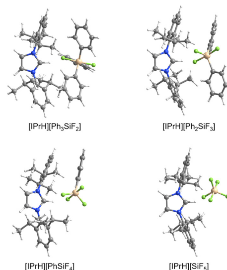
Fig. 8 Optimised structures of [\text{IPrH}][\text{Ph}_{4-n}\text{SiF}_{n+1}] ( n = 1\text{--}4 ).
