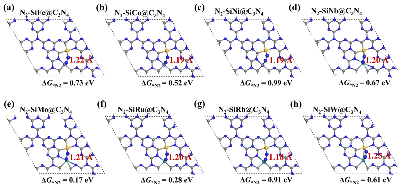
Fig. 3 (a–h) Side-on adsorption configurations of *\text{N}_2 on \text{SiM@C}_3\text{N}_4 with adsorption-free energies ( \Delta G_{*N_2} ) and N–N bond lengths. \text{N}_2 adsorption configuration on \text{SiRe@C}_3\text{N}_4 is shown in Fig. S4 (ESI†).
