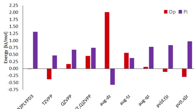
Fig. 2 Electronic energy differences for conformations in the methanol–furan complex with OH-bonded top Ot reference at different levels of theory. The left most left bar contains the only DFT results at B2PLYPD3/6-311++g(d,p)B3PLYPD3/6-311++g(d,p) level, all other energies refer to DLPNO-CCSD(T) energies. The capitalized basis sets are Ahlrichs def2-(T or Q)ZVPP and its extrapolation; the lower case basis sets are aug-cc-pv(d, t, or q)z basis sets and two extrapolations of them.
