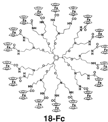
Fig. 10 Metallo-dendrimers with 3 ( 3-Fc ), 9 ( 9-Fc ) and 27 ( 27-Fc ) terminal amidoferrocenyl groups that recognize oxo-anions using cyclic voltammetry, CV (see Fig. 11). Reproduced with permission from ref. 100. Copyright 1997 American Chemical Society.
