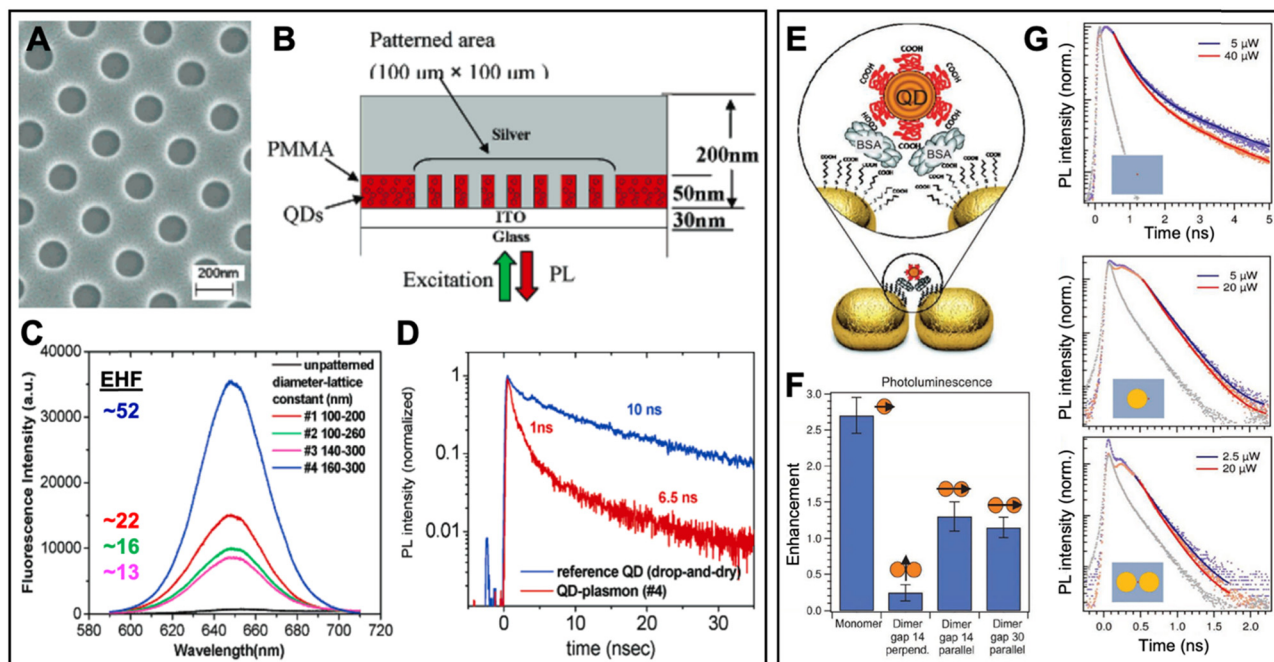
Fig. 8 Examples of surface-based metal–QD nano hybrids for PEF. (A) SEM image (top view) of a nanoarray of holes with diameters of \sim 160 nm and a lattice constant of \sim 300 nm in PMMA. (B) Schematic (side view) of the finished Ag–QD nanostructure. (C) QD PL spectra ( \lambda_{\text{ex}} = 532 nm) and EHF from arrays with different nanodisk diameters and lattice constants. (D) QD PL lifetime measurement of QDs ( \lambda_{\text{ex}} = 545 nm; \lambda_{\text{em}} = 655 nm) on a glass substrate (blue) and QDs in the 160 nm diameter and 300 nm lattice constant nanoarray (red). A to D adapted with permission from ref. 98. Copyright 2005 American Chemical Society. (E) PEG-coated QDs were precisely attached in the gap region of Au nanodisk dimers via binding to BSA. (F) Integrated PL EHF of different Au nanodisk monomer and dimer structures with different gap sizes and perpendicular or parallel excitation polarization. (G) PL decay curves ( \lambda_{\text{ex}} = 636 nm; \lambda_{\text{em}}: 650\text{--}690 nm) for QDs on the ITO substrate (top), a QD coupled to a Au nanodisk monomer (center), and a QD coupled to a dimer antenna with a 14 nm gap (bottom). The gray curves show the instrument response function. Note the different time scales for QDs alone and QDs coupled to Au nanodisks. (E–G) Adapted with permission from ref. 97. Copyright 2012 Wiley–VCH Verlag GmbH & Co. KGaA, Weinheim.
