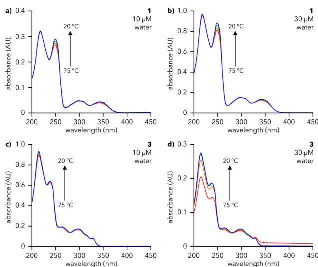
Fig. 2 UV-vis studies of 1 and 3 in solution. UV-vis spectra of (a) and (b) 1 and (c) and (d) 3 collected upon cooling aqueous solutions at the indicated concentrations from 75 ^{\circ}\text{C} (red line) to 20 ^{\circ}\text{C} (blue line) at 0.5 \text{ }^{\circ}\text{C min}^{-1} . Spectra were collected at 75, 60, 40, and 20 ^{\circ}\text{C} . Spectra in (a)–(c) were collected in a cuvette with path length ( l ) of 10 mm; spectra in (d) were collected in a cuvette with l = 1 mm.
