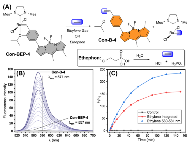
Fig. 3 (A) Reaction of Con-BEP-4 with ethylene gas or ethylene from ethephon hydrolysis. (B) Emission spectra of Con-BEP-4 exposed to ethylene. Timepoints represented are t = 0, 5, 10, 15, 20, 25, 30, 40, 50, 60, 75, 90, 105, 120, 150, and 180 min. Gray bar at 581 nm represents wavelength with maximum increase in emission intensity. (C) Normalized emission intensity of Con-BEP-4 control sample or treated with ethylene (integrated emission and 580–581 nm).
