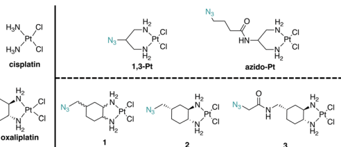
Fig. 1 Azide-functionalized cisplatin and oxaliplatin mimics used in this study.
