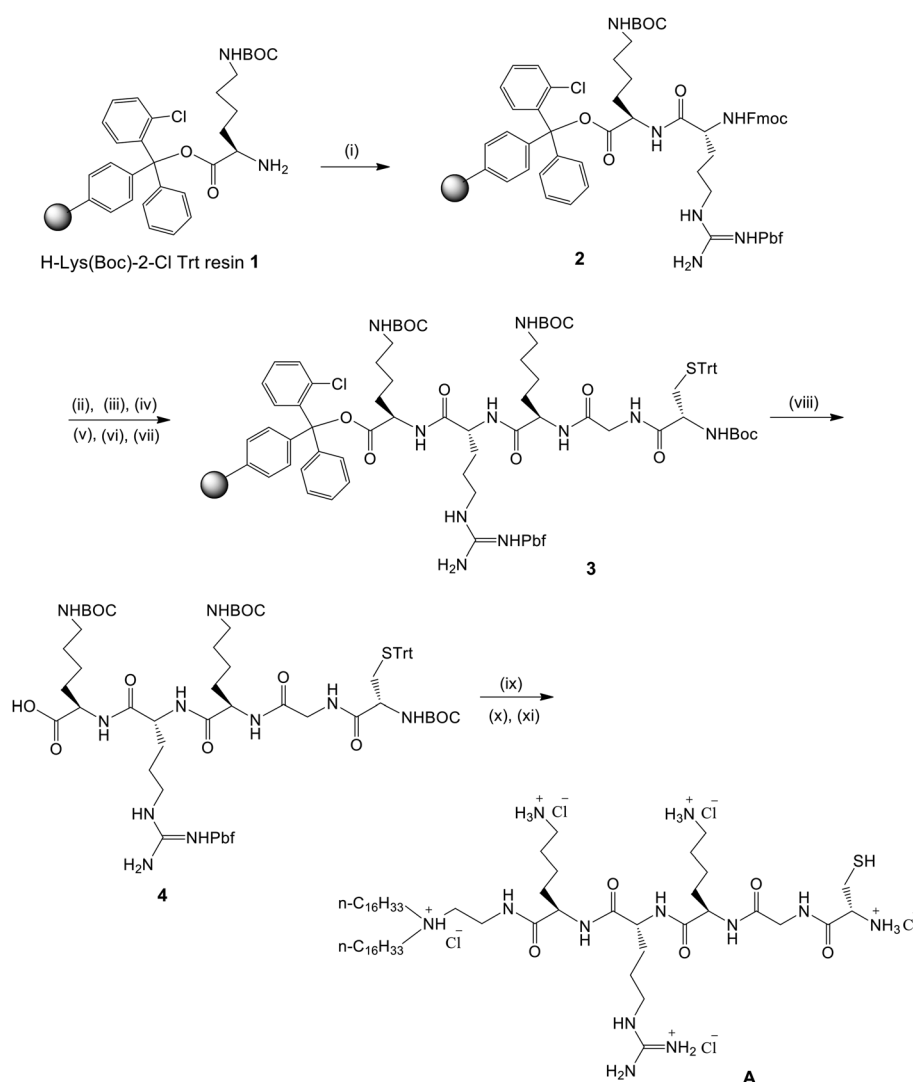
Fig. 2 Solid phase synthesis of the CGKRK-lipopeptide (CLP). Reagents: (i) Fmoc-Arg(Pbf)-OH (2 equiv.), HATU (2 equiv.), DIPEA (4 equiv.), rt, 1 \times 30 min, and then 1 \times 1 h (ii) piperidine-DMF (1 : 4), rt, 4 min, (x2); (iii) Fmoc-Lys(BOC)-OH (2 equiv.), HATU (2 equiv.), DIPEA (4 equiv.), rt, 1 \times 30 min, and then 1 \times 1 h (iv) piperidine-DMF (1 : 4), rt, 4 min, (x2); (v) Fmoc-Gly-OH (2 equiv.), HATU (2 equiv.), DIPEA (4 equiv.), rt, 1 \times 30 min, and then 1 \times 1 h; (vi) piperidine-DMF (1 : 4), rt, 4 min, (x2); (vii) BOC-Cys(Trt)-OH (2 equiv.), HATU (2 equiv.), DIPEA (4 equiv.), rt, 1 \times 30 min, and then 1 \times 1 h; (viii) TFA-Dry DCM (0.5%), 2 h, 0 °C; (ix) N,N -di- n -hexadecyl- N -2-aminoethylamine, dry DCM, EDCl, HOBT, 12 h; (x) TFA-thioanisole-ethanedithiol-anisole (90 : 5 : 3 : 2), 3 h, 0 °C; and (xi) \text{Cl}^- ion exchange (Amberlyst resin).
