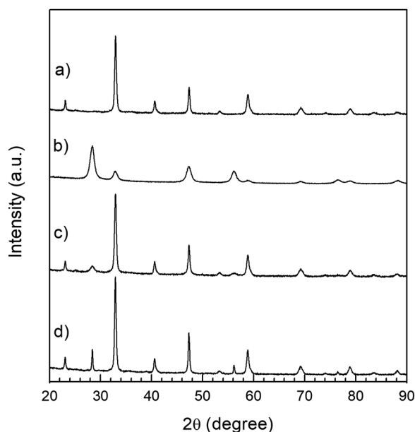
Fig. 3 XRD patterns. (a) LSC nanoparticles; (b) GDC powder with particles of spherical shape; (c) LSC75-GD MW 25 cathode before the sintering process; (d) LSC75-GD MW 25 cathode after 2H at 850 °C.
