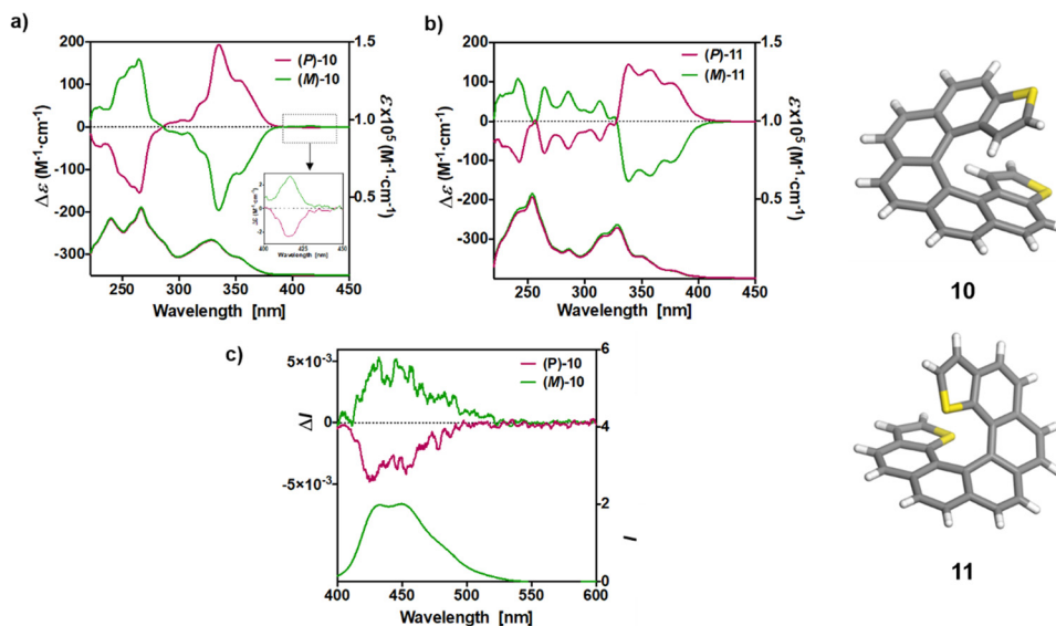
Fig. 3 The experimental UV-vis (bottom) and ECD (top) spectra of the ( P ) and ( M ) isomers of 10 and 11 ( \text{CH}_2\text{Cl}_2 , C \sim 10^{-5} M) are shown in panels (a) and (b), respectively. The inset in (a) shows the magnified ECD of ( P ) and ( M )- 10 in the 400–450 nm region. The fluorescence (bottom) and CPL (top) spectra of ( P ) and ( M )- 10 are shown in panel (c).
