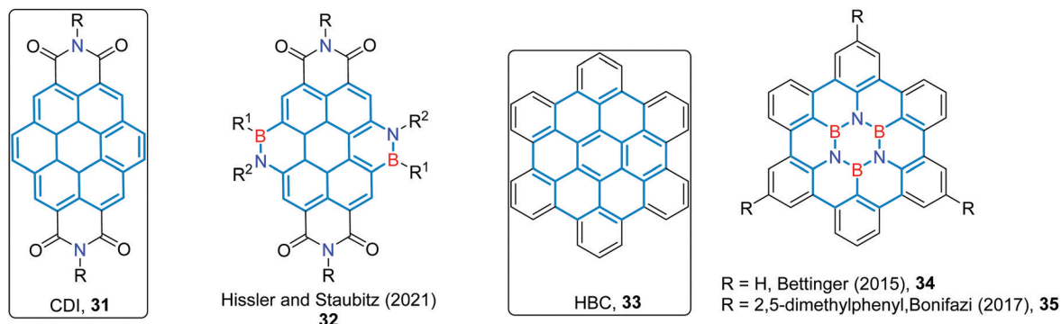
Fig. 10 Multi-BN-doped CDI, HBC and their derivatives.
