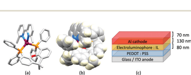
Fig. 7 The structure of the [Cu(xantphos)(6,6'-Me 2 bpy)] + cation in the [PF 6 ] - salt (CSD refcode GABVAJ): (a) with H atoms omitted, and (b) in space-filling representation to show the steric shielding of the Cu(i) centre. (c) Architecture of the LEC devices containing [Cu(xantphos)(N ^ N)][PF 6 ] with N ^ N = 6-Mebpy, 6-Etbpy or 6,6'-Me 2 bpy. IL = [EMIM][PF 6 ], and Cu-iTMC: IL molar ratio = 4:1.
