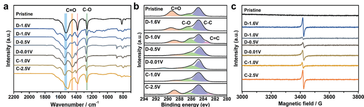
Fig. 5 Ex situ (a) FT-IR spectra, (b) XPS C 1s spectra and (c) EPR spectra of the Ni-DHBQ electrode recorded at different potentials.
