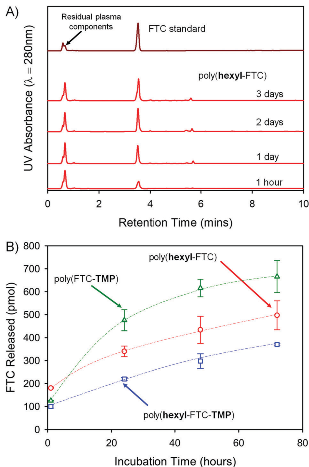
Fig. 5 HPLC studies of FTC release from powdered FTC-containing polymers of differing architectures. (A) Demonstration of the appearance of FTC parent drug on exposure of linear poly( hexyl -FTC) to mixed gender human plasma; (B) comparative cumulative release of FTC from linear poly( hexyl -FTC) (open red circles), branched poly( hexyl -FTC-TMP) (open blue squares), and crosslinked poly(FTC-TMP) (open green triangles).
