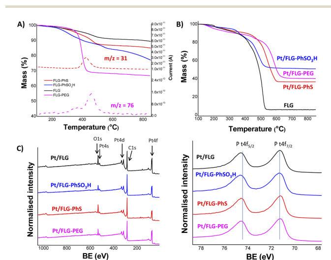
Fig. 1 Characterisation of functionalised graphene samples. (A) TGA-MS under N 2 of functionalised graphene samples. Phenyl and PEG fragments m/z 76 (C 6 H 4 + ) and m/z 31 (CH 3 O + ), respectively. (B) TGA under air of platinum supported graphene samples. (C) XPS spectra of platinum supported graphene samples (left panel) and platinum Pt 4f component (right panel).
