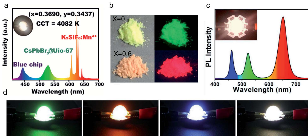
Fig. 8 (a) PL spectra of the as-fabricated WLEDs with the CsPbBr_3@Uio-67 composite and commercial K_2SiF_6:Mn^{4+} red phosphor deposited on the blue chip (InGaN, 455 nm). Inset: Photograph of the WLEDs. (b) Photographs of CsPb_{3-x}Br_x/MOF-5 powders ( x = 0 and 0.6 ) taken under daylight (left) and 365 nm UV illumination (right). Reprinted with permission from ref. 113. Copyright 2019 American Chemical Society. (c) The corresponding EL spectrum with a photo of the white LED in the inset. Reprinted from ref. 112. Copyright 2019, with permission from Elsevier. (d) Photograph of blue, green, red, and white LEDs, respectively, using Bio-MOF-1 developed by Zhang et al. Reprinted from ref. 108. Copyright 2019, with permission from Elsevier.
