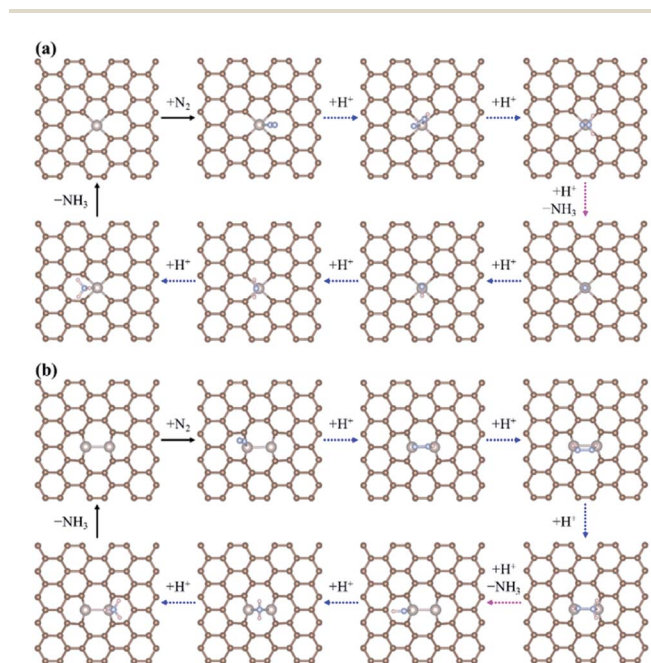
Fig. 2 The optimized geometric structures of N_2RR intermediates along the most favourable reaction pathway on (a) the Ru SAC and (b) the homo- Ru_2 DAC.
