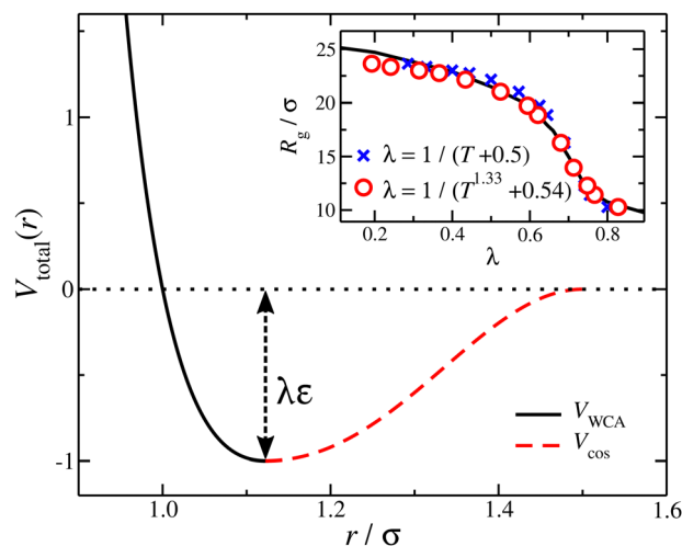
Fig. 1 The non-bonded, bead-bead interaction potential V(r) with \lambda = 1 , showing the contributions from V_{\text{WCA}}(r) + V_{\text{SW}}(r) (black) and V_{\text{cos}}(r) (red). Inset: Average radius of gyration of a nanogel particle via \lambda variation (black line) and temperature T variation (symbols). Two relations between \lambda and T are presented.
