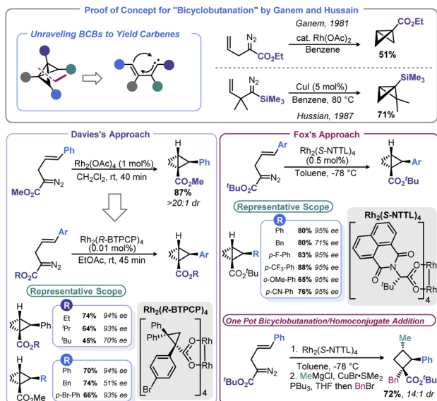
Scheme 3 BCB synthesis via metal-mediated intramolecular [2 + 1] bicyclobutane.
