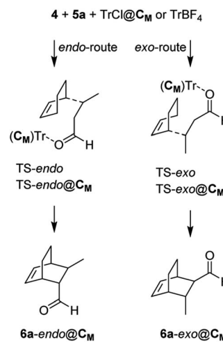
Scheme 2 Endo and exo routes for the in silico studies of the model DA reactions and nomenclature adopted: TS-endo and TS-exo refer to the reaction with \text{TrBF}_4 , while TS-endo@ C_M and TS-exo@ C_M refer to the reaction with \text{TrCl} and the capsule.
