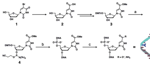
Scheme 1 Synthesis of DNA strands containing Im OC or Im OA nucleotides. The DMTr-modified nucleoside 3 was synthesised by the reported procedure. 55 (a) 2-Cyanoethyl N,N -diisopropylchlorophosphoramidite, DIPEA, CH 2 Cl 2 , rt, 0.5 h (78%); (b) DNA synthesiser; (c) 0.3 M NaOH aq., 37 °C (for Im OC ) or 25% ammonia aq., 55 °C (for Im OA ). DMTr = 4,4'-dimethoxytrityl.
