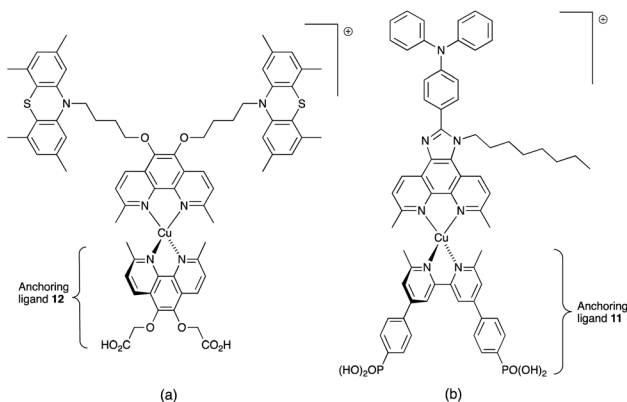
Scheme 16 The structures of (a) [\text{Cu}(12)(\text{tmpDMP})]^+ reported by Ashbrook and Elliott, and (b) a copper(I) dye reported by our group tested with a \text{Co}^{3+}/\text{Co}^{2+} redox mediator. Both heteroleptic dyes were assembled in situ using the SALSAC approach.
