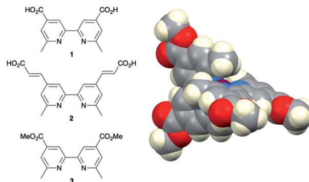
Fig. 7 Structures of ligands 1–3, and the structure of [\text{Cu}(3)]^+ in the [\text{PF}_6]^- salt (CSD refcode JOHXIO). The space-filling representation is used to emphasize the protection imparted by the 6- and 6'-methyl groups.
