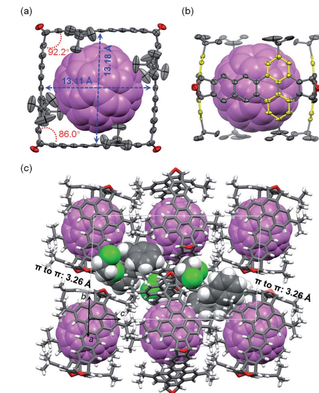
Fig. 6 Crystal structure of C_{60} \subset 3 \cdot 2(C_2H_4Cl_2) \cdot 2(C_6H_5CH_3) : (a) top view of C_{60} \subset 3 ; (b) side view of C_{60} \subset 3 ; (c) molecular packing in a unit cell. C_{60} is shown in violet with a space-filling model; in panels a and b, carbon and oxygen atoms in 3 are shown as ellipsoids at the 50% probability level, and hydrogen atoms are removed for clarity; in panel c, molecules of 3 are shown with stick models, and co-crystallized solvent molecules are shown with space-filling models.
