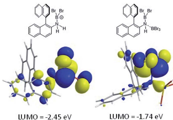
Fig. 4 LUMO of, left, borinium cation G formed on protonation of an aminoborane, right, borinium equivalent F formed on addition of BBr 3 .
