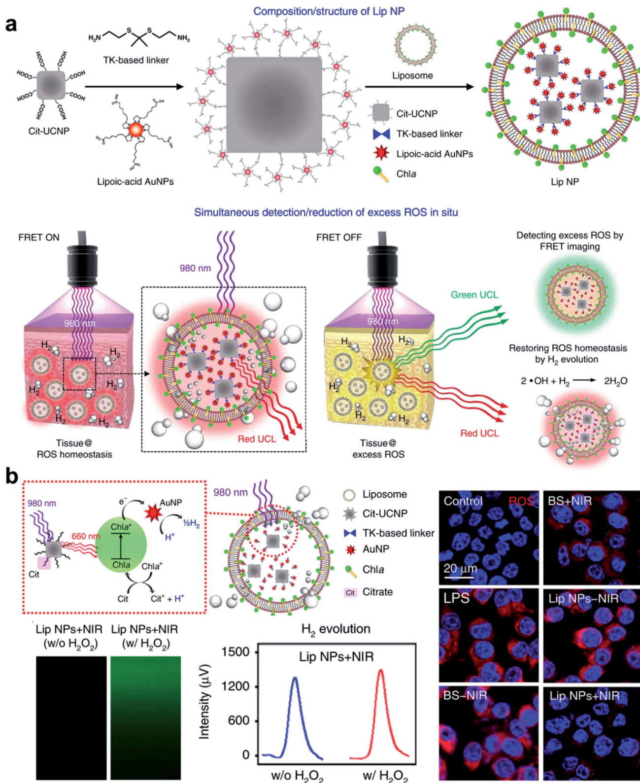
Fig. 5 UCNP-based nanocomposites for \text{H}_2 gas therapy. (a) Photosynthesis-inspired \text{H}_2 generation using a chlorophyll-loaded liposomal UCNP-based nanoplatform to (b) detect and scavenge excess ROS. 42 Adapted from ref. 42 with permission from Nature Publishing Group, copyright 2020.
