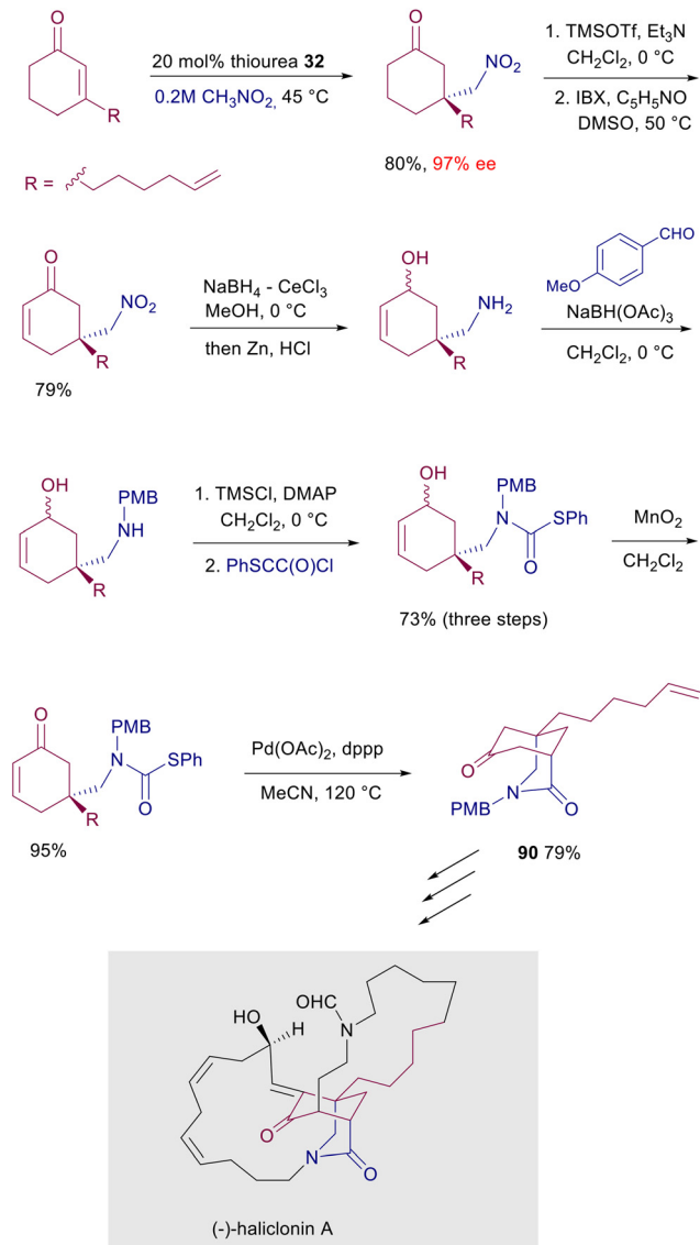
Scheme 68 Synthesis of the macrocyclic alkaloid ( - )-haliclونin A.
