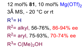
Scheme 59 Enantioselective conjugate addition of nitroalkanes to enones using Mg(II)-complexes.
