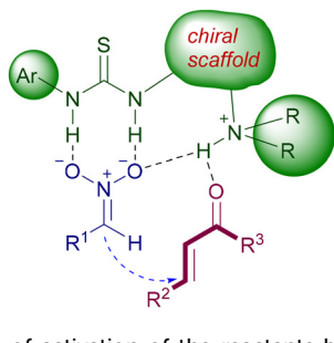
Fig. 3 Mechanism of activation of the reactants by chiral bifunctional thioureas.
