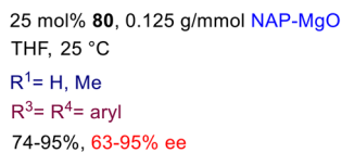
Scheme 59 Enantioselective conjugate addition of nitroalkanes to enones using Mg(II)-complexes.
