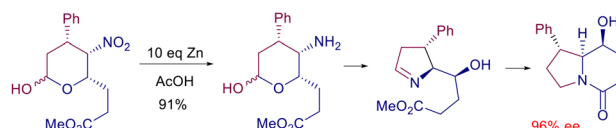
Scheme 14 Synthesis of nitrolactols and their application to the preparation of optically active indolizines.
