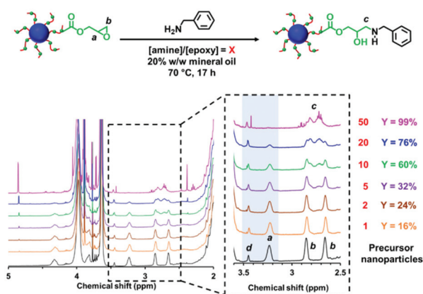
Fig. 2 ^1\text{H} NMR spectra recorded in \text{CD}_2\text{Cl}_2 for \text{P(LMA}_{50}\text{-stat-GlyMA}_9\text{)-PMMA}_{67} before (black spectrum) and after reaction with benzylamine at 70 °C for 17 h at 20% w/w solids when using an [amine]/[epoxy] molar ratio (X) of 1 (orange spectrum), 2 (brown spectrum), 5 (purple spectrum), 10 (green spectrum), 20 (blue spectrum) and 50 (pink spectrum), respectively. Expansion of the 2.5–3.6 ppm region confirms the systematic loss of epoxy groups (note the gradual attenuation of methine signal a and the evolution of a new methylene signal c on increasing the [amine]/[epoxy] molar ratio). In each case, the epoxy loss (Y%) was determined by comparing the satellite signal d assigned to the PMMA backbone at 3.43–3.47 ppm to the methine signal a corresponding to the epoxide ring at 3.12–3.30 ppm.
