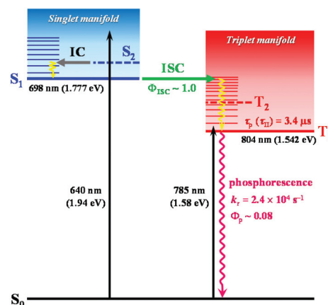
Fig. 4 Excited state deactivation pathway and related photophysical parameters for the Au 25 -rod in deaerated THF. The vertical transition energy from S_0 to S_1 or T_1 obtained from theoretical calculations is also shown. The S_2 and T_2 states theoretically predicted to exist in the energetic vicinity of the S_1 and T_1 states (Fig. S11†) are shown as dashed lines.
