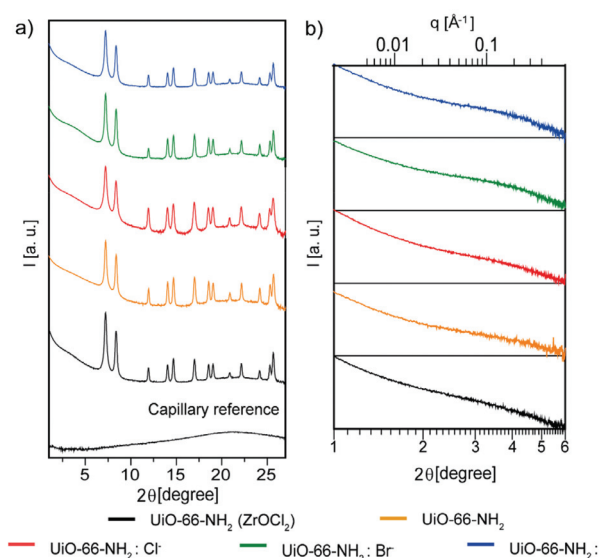
Fig. 3 Crystallographic characterization of UiO-66- NH_2 NMOFs: UiO-66- NH_2 ( ZrOCl_2 ) (black), UiO-66- NH_2 (orange), UiO-66- NH_2:Cl^- (red), UiO-66- NH_2:Br^- (green) and UiO-66- NH_2:I^- (blue). (a) WAXS analysis measured at a sample-to-detector distance of 288 mm and (b) SAXS analysis measured at a sample-to-detector distance of 1343 mm in capillary mode.
