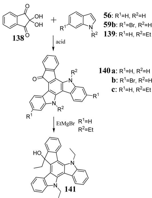
Scheme 46 Synthesis and reactivity of 5,10-diazatruxen-15-ones.
