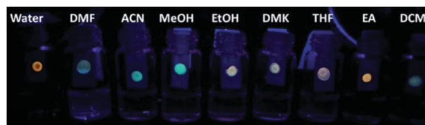
Fig. 6 Images of paper sensor strip containing CNPs after exposure to the vapor of solvents taken under a UV lamp (365 nm) (reproduced with permission from RSC Adv. , 2016, 6, 83501–83504, Copyright 2016, The Royal Society of Chemistry).
