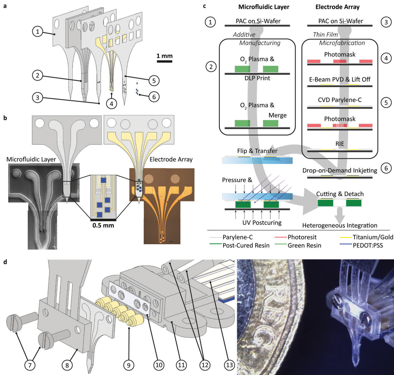
Fig. 1 Hybrid fabrication of the multimodal intracranial implant: (a) exploded view of the implant (1 to 6) and assembled headstage for acute in vivo experiments (7 to 13): 1 bottom PAC layer (2 \mu\text{m} ), 2 3D printed, flexible body with microfluidic system (200 \mu\text{m} ), 3 middle PAC layer (2 \mu\text{m} ) with \mu -fluidic in- and outlet, 4 10 nm titanium-100 nm gold electrodes 5, top PAC layer (2 \mu\text{m} ) with etched \mu -fluidic in- and outlets as well as electrical contacts, 6 Drop-on-demand inkjet-printed PEDOT:PSS layer (77 \pm 11 nm), 7 fastener M0.6 \times 5 mm, 8 3D printed socket for acute in vivo experiments, 9 pogo pins, 10 medical-grade double-sided adhesive tape (85 \mu\text{m} ), 11 3D printed fluidic and electric interface with M0.6 thread, 12 1/32" polyethylene tubing (0.8 mm OD, 0.4 mm ID) and 13 tailored FPC cable (5 ways, 1 mm pitch); (b) left: technical drawing and SEM picture of 3D printed body showing the \mu -fluidic channels (top view) and right: technical drawing and optical micrograph of the Au layer (top view). (c) Convergent hybrid fabrication schema, combining additive manufacturing and thin-film microfabrication; (d) exploded view and microscopy picture of the assembly.
