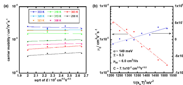
Fig. 8 (a) Hole mobilities plotted for the square root of the electric field at various temperatures in the N* phase of the compounds 1–3 mixture (low temperature region). (b) Plots of zero-field mobility \mu_0 and \beta as a function of the square of 1/k_B T in the N* phase of the LC mixture (low temperature region).
