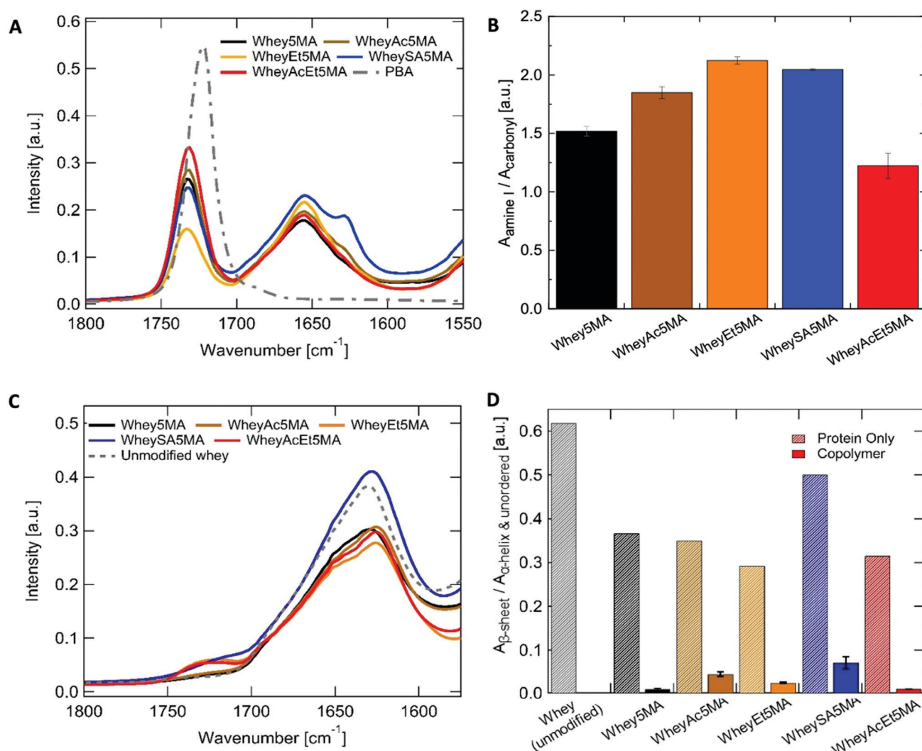
Fig. 3 (A) ATR-FTIR spectra of the copolymer (WPI : BAC : n -BA, 25 : 25 : 50) expected based on feed) and poly( n -BA) homopolymer. (B) Ratios between protein and poly( n -BA), measured as area ratios of the protein amide I band (centered at 1647\text{ cm}^{-1} ) to the poly( n -butyl acrylate) carbonyl peak (centered at 1737\text{ cm}^{-1} ), n = 3 . (C) ATR-FTIR spectra of protein powder before and after charge modifications and methacrylation. (D) Amide I band in the protein powder and copolymer spectra deconvoluted to obtain ratio of the low frequency ( \sim 1630\text{ cm}^{-1} , \beta -sheet) to the high frequency component ( \sim 1652\text{ cm}^{-1} , \alpha -helix and unordered structures). N = 1 for protein powders, N = 5 for copolymers.
