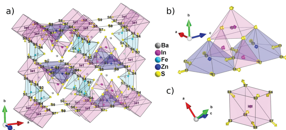
Fig. 3 Representation of the centrosymmetric ( Amm ) hypothetical aristotype of \text{Ba}_5\text{ZnFe}_2\text{In}_4\text{ZnS}_{15} and the atomic shifts necessary to derive the real structure. The arrows representing the atomic displacements are drawn to scale meaning that the tip of the arrows points to the real position of the atoms. The position identification refers to the Ama2 cell. (a) Whole cell, (b) T2 super-tetrahedral subunit and (c) coordination sphere of In1.
