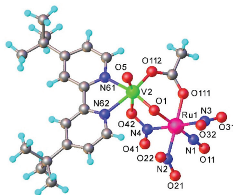
Fig. 7 X-ray diffraction structure of [Ru(NO)(NO 2 ) 2 (μ-NO 2 )(μ-CH 3 COO)(μ-O)VO(L)], where L = 4,4'-di- tert -butyl-2,2'-bipyridyl. The structure is taken from those reported on the CSD; code: FAFMEI.
