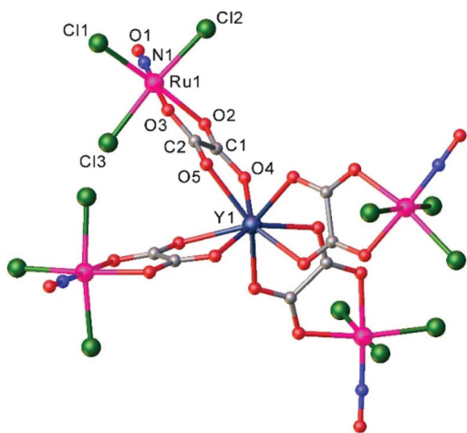
Fig. 6 X-ray diffraction structure of the complex anion [Ln(RuCl 3 (μ-C 2 O 4 )(NO)) 4 ] 5- . The structure is taken from those reported on the CSD; code: YUWLEJ.
