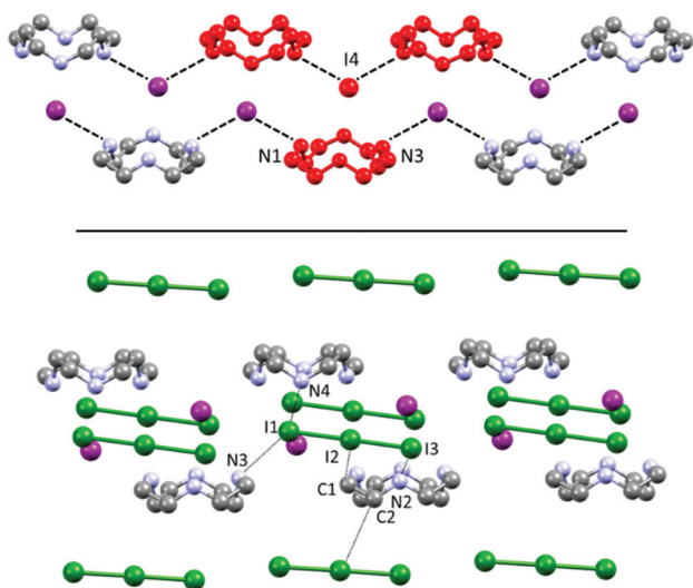
Fig. 3 Top: Visualization of H-bonded (\text{H}_2\text{Cyclen}\cdot\text{I})_n^{n+} polycationic ribbons, repeating unit (red), as discussed in Fig. 2. Bottom: Their interaction with \text{I}_3^- counteranions surrounding and spacing such ribbons.
