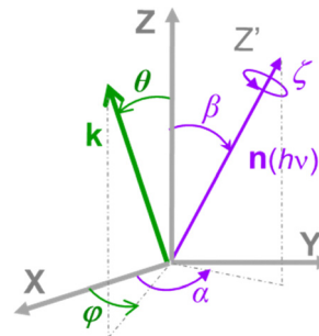
Fig. 1 Schematic of the Euler angles (\alpha, \beta, \zeta) defining the rotation of the molecular frame (X,Y,Z) into the laboratory frame (X',Y',Z'), where the Z' axis lies along the light quantization axis n(h\nu) , linear polarization E or propagation axis of elliptically polarized light, and the polar and azimuthal angles (\theta, \varphi) defining the orientation of the photoelectron momentum k in the MF.
