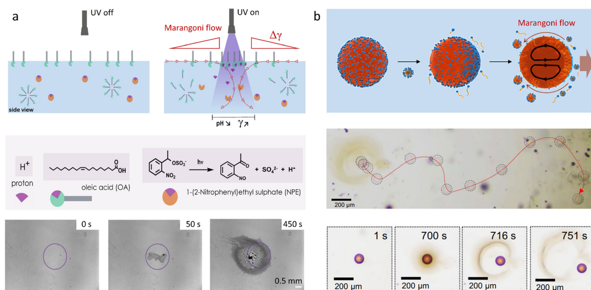
Fig. 10 (a) Self-sustained Marangoni flow at a 2D air–water interface, triggered by local UV exposure. Photoacid generator 1-[(2-nitrophenyl)ethyl]sulphate (NPE sulfate) produces an acid, which protonates the surfactant oleate. Thereby, the surface tension increases at the site of UV exposure, where phase separated oleic acid droplets accumulate. Adapted from ref. 137 with permission from the Wiley–VCH publishing group, Copyright 2021. (b) Propulsion of octanol droplets in an aqueous solution ( i.e. 3D system): an asymmetric occupation of lipid (of which the formation is catalyzed by the octanol–water interface) at the droplet interface results into an internal Marangoni flow in the droplet, which drives their propulsion. Adapted from ref. 147.
