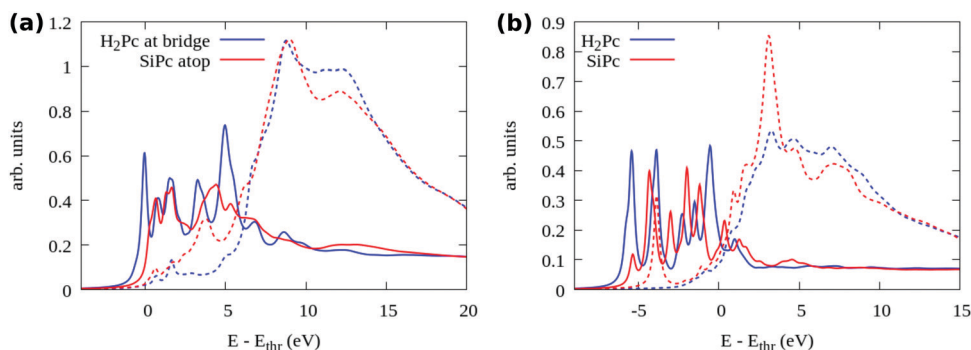
Fig. 9 Comparison of the simulated N 1s NEXAFS between (a) bridge H_2Pc/6H-SiC(0001)-(3 \times 3) and top 6H-SiC(0001)-(3 \times 3) , (b) gas phase H_2Pc and SiPc. The solid lines represent photon polarization along the surface normal and the dotted ones in the surface plane.
