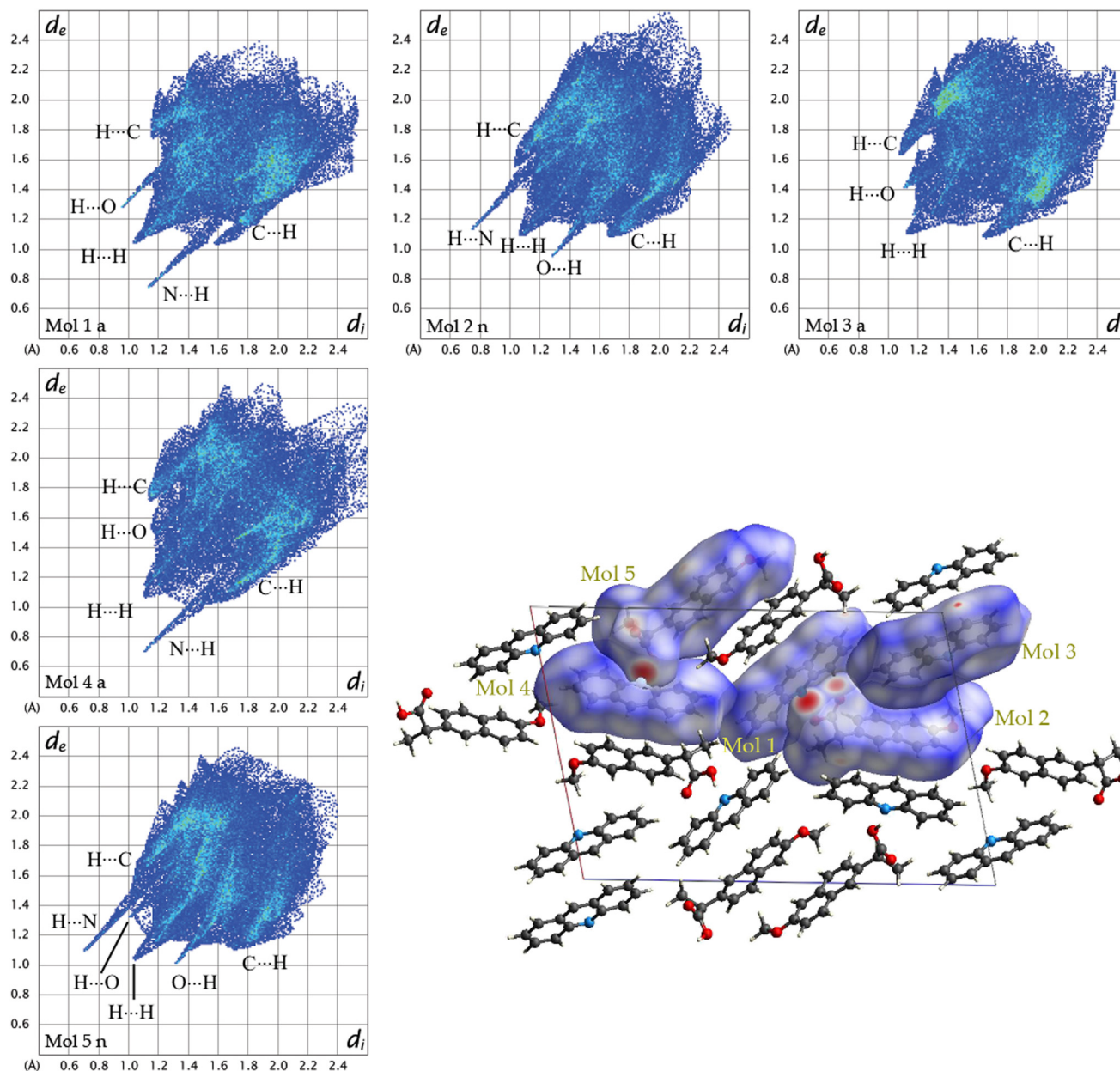
Fig. 6 Fingerprint plots for each symmetry-independent molecule in 1α and crystal structure model of 1α viewed along the b -axis showing Hirshfeld surfaces with d -norm plotted.
