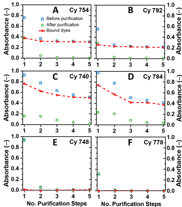
Fig. 2 Absorption peak intensity variations for MeOH solutions of NaGdF 4 :Yb,Er UCNCs with Cy 754 (A), Cy 792 (B), Cy 740 (C), Cy 784 (D), Cy 748 (E), and Cy 778 (F) dyes. The initial dye concentrations are similar in all the experiments (3 \mu\text{g ml}^{-1} ). The blue square symbols show the absorption intensities of MeOH solutions before each purification step, which contain both bound and unbound dyes. The green circle symbols are related to the absorption intensities of the supernatant solutions that contain the unbound dyes. The red dashed curves are obtained by subtraction of the green from the blue values and show the absorption caused by the bound dyes.
