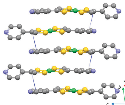
Fig. 18 Details in the crystal structure of [\text{Ni}(\text{4-pedt})_2] molecular head-to-tail stacking, viewed parallel to the central molecular plane.
