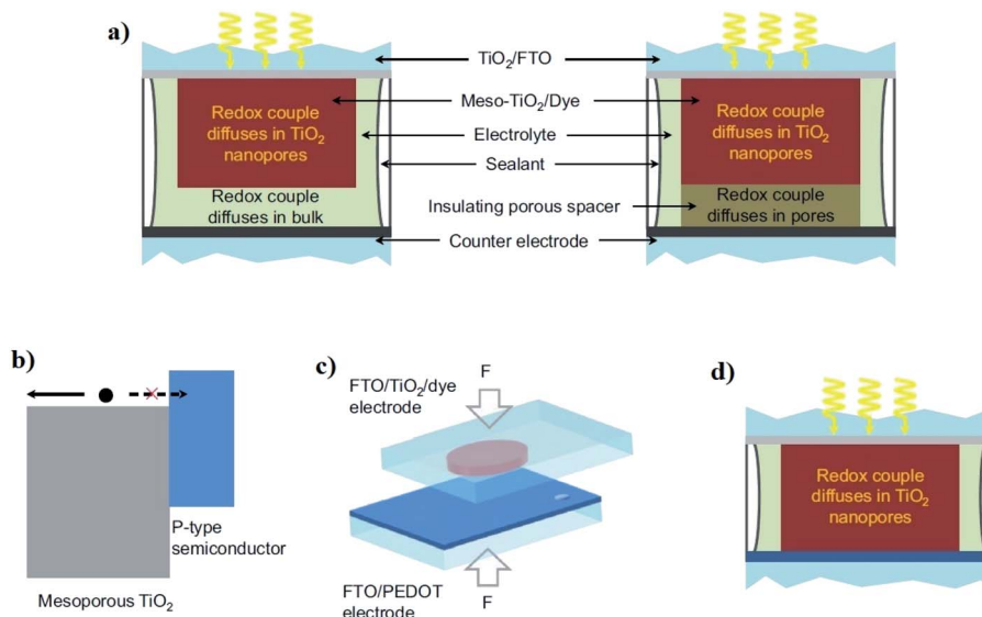
Fig. 3 (a) Traditional DSSC use either a thermoplastic or porous insulating spacer to avoid short circuit between the mesoporous TiO 2 and the counter electrode. (b) Type II junction alignment 31 of the band edges for the mesoporous TiO 2 film and a p-type semiconductor layer. The p-type semiconductor serves as an electron-blocking hole-selective charge collection layer. (c) The sensitized TiO 2 electrode and the PEDOT semiconductor-based counter electrode make direct contact via mechanically pressing and make a new DSSC embodiment. (d) In the DSSC with the contacted electrodes, the redox couple diffuses merely through the mesoscopic TiO 2 film (reproduced from reference with permission 25 ).
