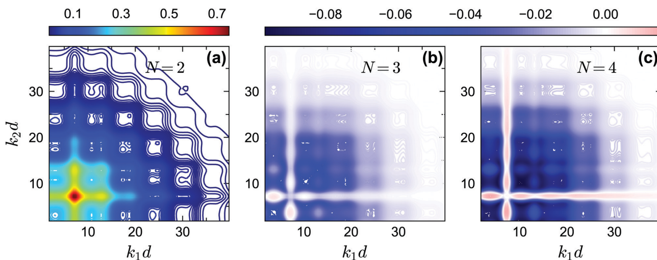
Fig. 14 (a) The non-ergodicity parameters f_2^c(k_1, k_2) as a function of wavenumbers k_1 and k_2 at the critical packing fraction for closure level N = 2 ( i.e. , standard MCT) at \theta = 0.2 . The patterns of f_2^c(k_1, k_2) from N = 3 and N = 4 are similar. (b) The difference of the non-ergodicity parameters f_2^c(k_1, k_2) of closure level N = 3 with respect to the factorization approximation f_1^c(k_1) \times f_1^c(k_2) at the same state. (c) Same as in (b) but for N = 4 . The packing fractions are the same as in Fig. 5.
