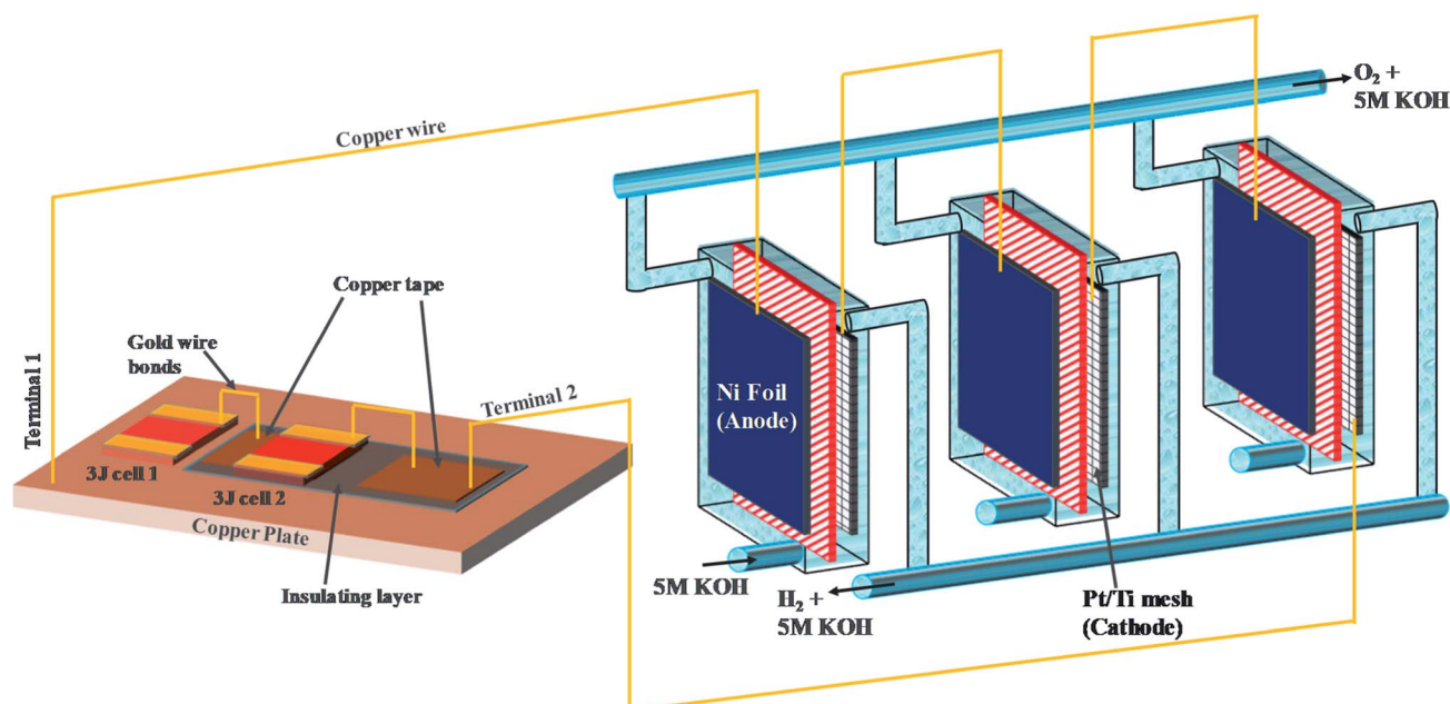
Scheme 1 The PV-electrolysis setup consists of two-3J CPV cells (each is composed of GaInP/GaInAs/Ge CPV cells ( 3.0 \times 3.0 \text{ mm}^2 )) connected in series to three alkaline electrolyzers, also connected in series. Each alkaline electrolyzer is composed of ca. 10 nm Pt particles deposited on both sides of a Ti mesh (Pt/Ti mesh) as the cathode and a \text{Ni}(\text{OH})_2/\text{Ni} as the anode. The electrolyte (5 M KOH solution) is recirculated. Terminal 1: back side of the cells (+), and terminal 2: front side of the cell (–). Light at 41-sun concentration illuminated the cells, without the use of Fresnel lenses.
