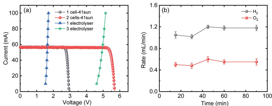
Fig. 2 (a) I - V curves of one (grey) and two 3J CPV cells (red) connected in series under 41-sun illumination overlapped with I - V curves of single (blue) and three (green) alkaline electrolyses connected in series. (b) \text{H}_2 and \text{O}_2 production rates from three alkaline electrolyses connected in series. Power is supplied from two CPV 3J cells connected in series under 41-sun illumination (without the use of Fresnel lenses to minimize further losses) as shown in Scheme 1.
